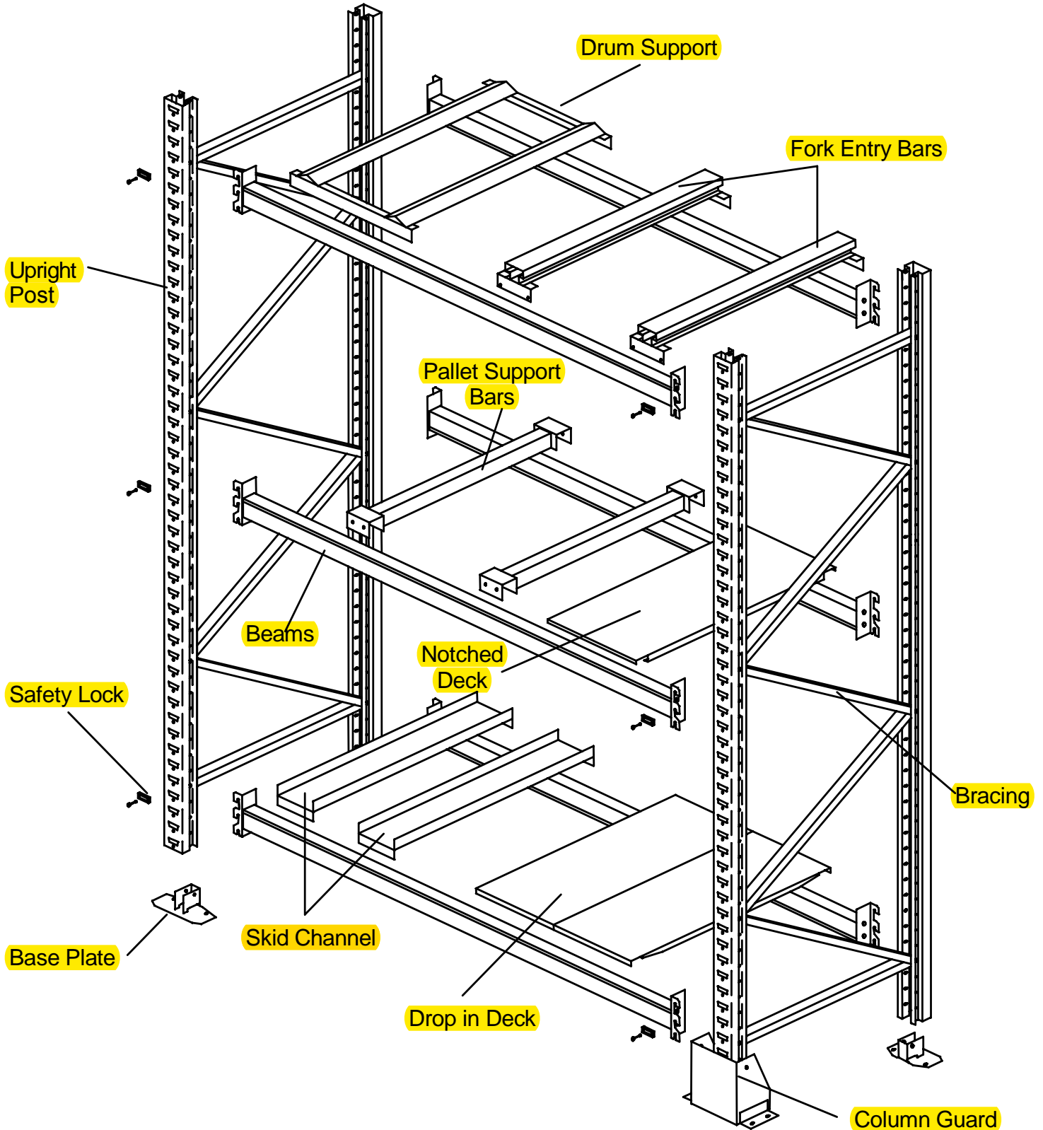
APEX Adjustable Pallet Racking
